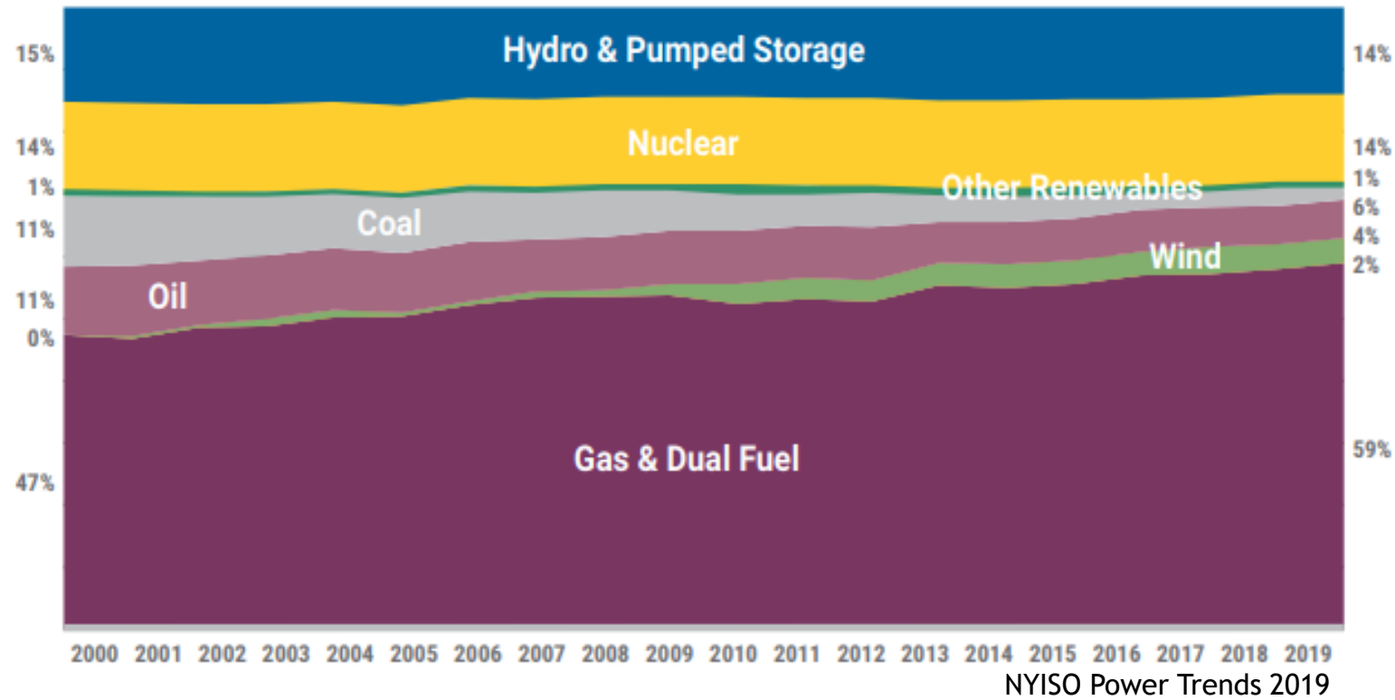
Figure 20: New York State Fuel Mix Trends: Capacity 2000-2019
